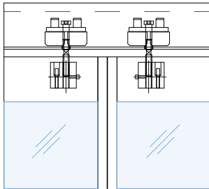
Detail D5:
