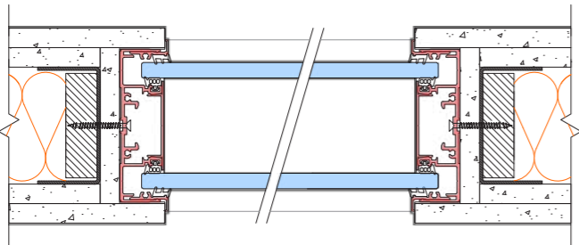
Horizontal section
