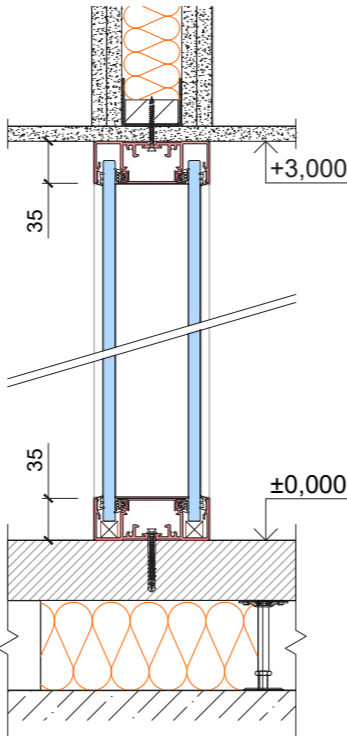
Vertical section
