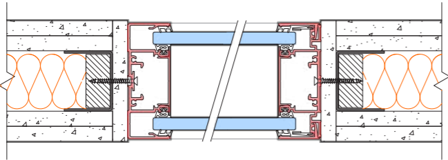
Horizontal section
