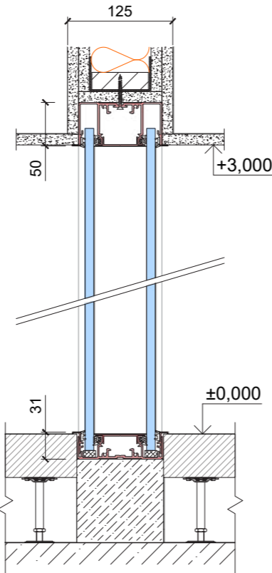
Vertical section
