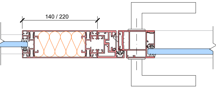
var. 2: IP140 / IP220 design
