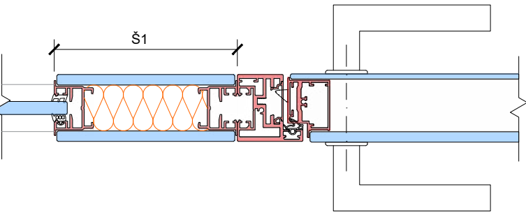
var. 1: IP double-glass
