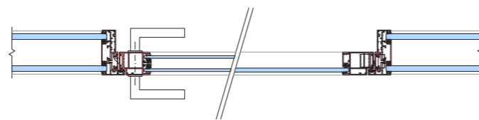
Framed Glazed Type UP Rw = 35-43 dB
