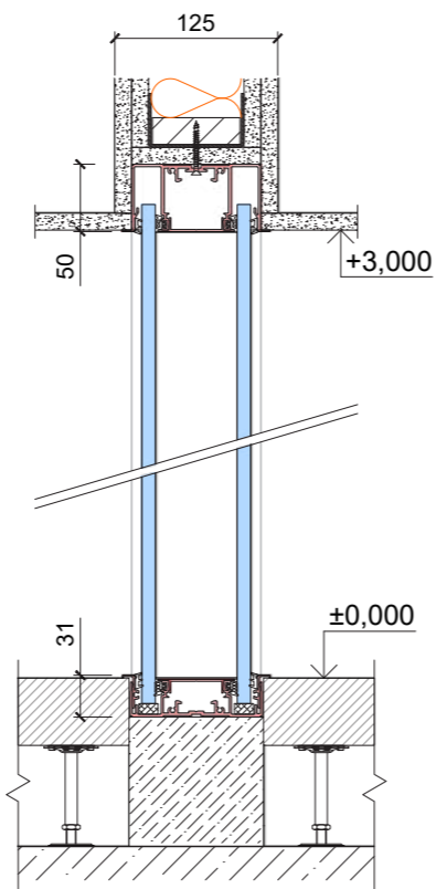
Vertical section
