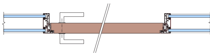
Wooden Rw = 32-40 dB
