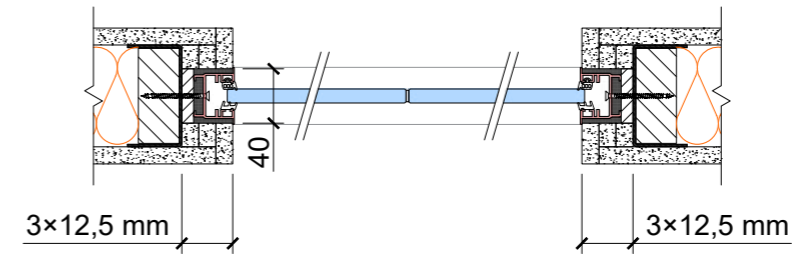
Horizontal section
